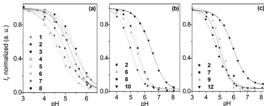
Figure 4. Comparative graphs of normalized maximum emission intensity as a function of pH for different pseudopeptidic fluorescent probes. Sample preparation: 2 \mu\text{M} , \text{H}_2\text{O} , 0.2% DMSO, universal buffer (0.04 M), NaCl (0.1 M): (a) compounds 1–8; (b) compounds 2, 6, 8, and 10; (c) compounds 2, 7, 9, and 12.
