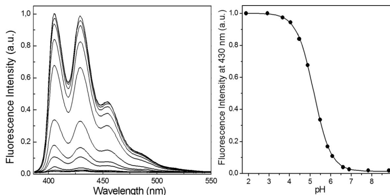
Figure 3. (a) Emission spectra of 1 as a function of the pH. (b) Intensity at the maximum emission of 1 as a function of pH. Experimental conditions: 2 μM of 1 , H 2 O (0.2% DMSO), universal buffer (0.04 M), NaCl (0.1 M); \lambda_{\text{exc}} = 374 nm.
