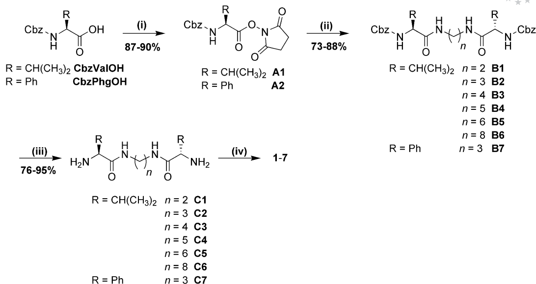
Scheme 2. General methodology for the preparation of macrocycles 1-7 . Reagents and conditions: (i) N -hydroxysuccinimide, DCC, THF; (ii) 1, n -alkanediamine, DME, RT; (iii) HBr/AcOH 33% followed by NaOH treatment; (iv) 9,10-bis(bromomethyl)anthracene, dry K 2 CO 3 , anhydrous CH 3 CN, reflux, chromatographic purification.
