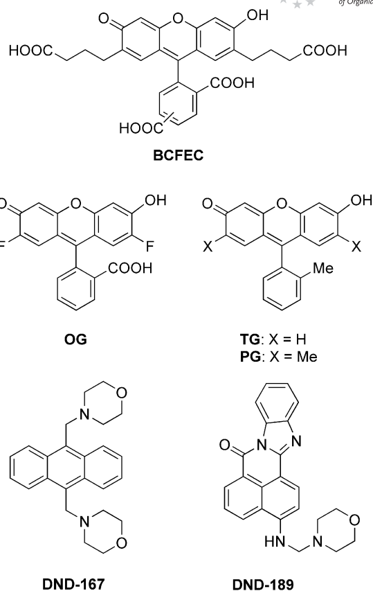
Scheme 5.
