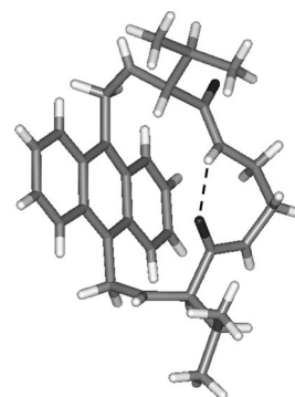
Figure 1. Molecular structure of macrocycle 1 obtained by X-ray diffraction showing the intramolecular hydrogen bond.
