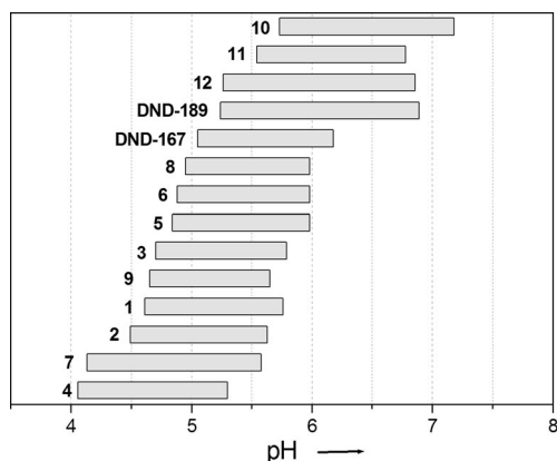
Figure 5. pH range for which a change in fluorescence emission from 20 to 80% takes place for the different sensors (2 \mu M, 0.2% DMSO in H 2 O).
