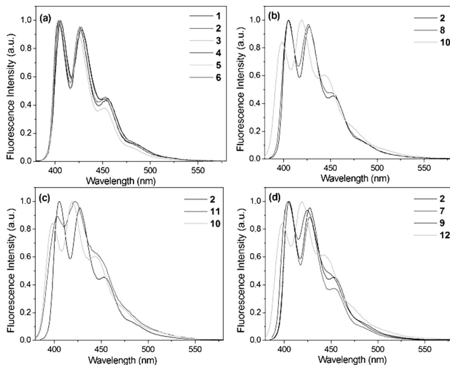
Figure 2. Comparative normalized emission spectra of synthesized anthracene derivatives in \text{H}_2\text{O} (0.02% DMSO at pH = 3.00). (a) Anthracenophanes 1–6 with different numbers of methylenic groups in the aliphatic bridge. (b) Anthracene derivatives 2 , 8 , and 10 with different numbers of pseudopeptidic chains in the structure. (c) Anthracenic derivatives 2 , 10 , and 11 with different substituents in the chemical structure. (d) Anthracene derivatives 2 , 7 , 9 , and 12 with different side-chains in the amino acid unit and different numbers of pseudopeptidic chains in the structure.
