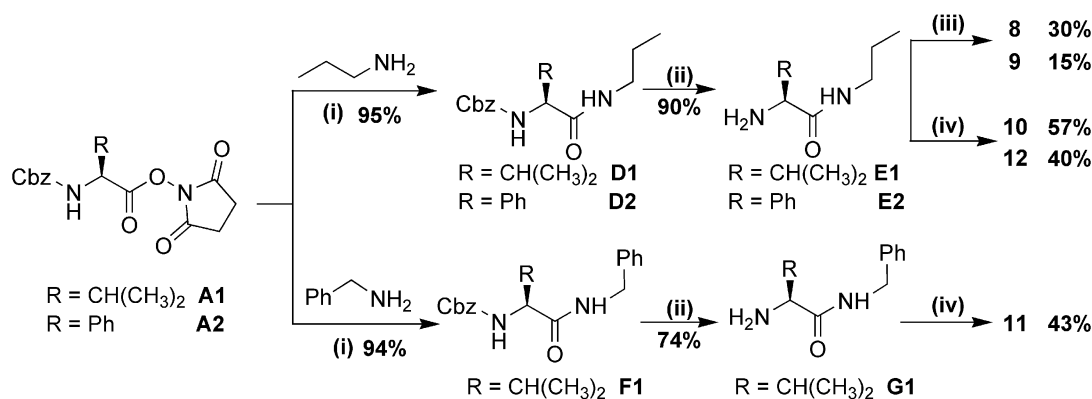
Scheme 3. General methodology for the preparation of open-chain pseudopeptides 8-12 . Reagents and conditions: (i) THF, reflux; (ii) HBr/AcOH 33% followed by NaOH treatment; (iii) 9,10-bis(bromomethyl)anthracene, anhydrous CH 3 CN, dry K 2 CO 3 , reflux; (iv) 9-(chloromethyl)anthracene, anhydrous CH 3 CN, dry K 2 CO 3 , reflux.
